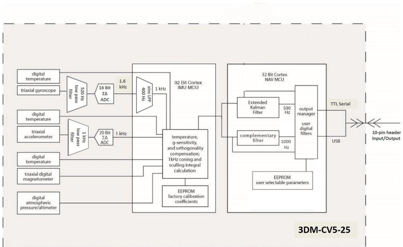
Figure 14 -3DM-CV5-25 Block Diagram
