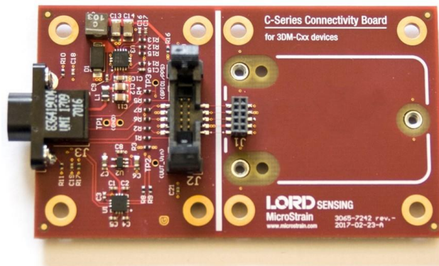
Figure 40 -C-Series Connectivity Board
