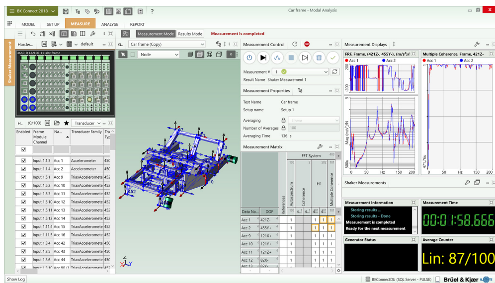
Fig. 1 Shaker Measurement task with easy setup and monitoring of time and frequency functions
