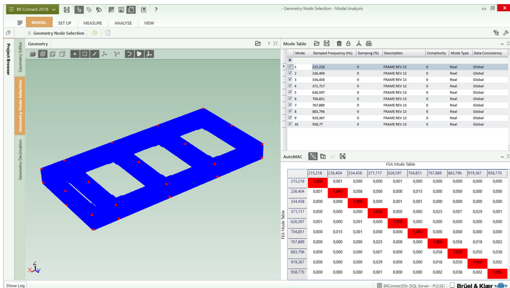
Fig. 3 Geometry Node Selection. By selecting nodes on an FE model, you can investigate how the AutoMAC builds up for the reduced geometry consisting of the selected nodes (highlighted)
