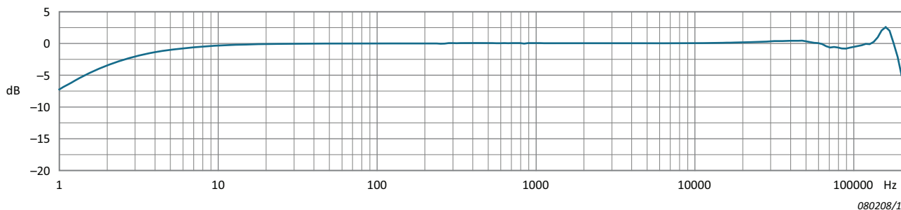
Fig. 1 Typical frequency response of Type 4138 recorded by means of the electrostatic actuator method
