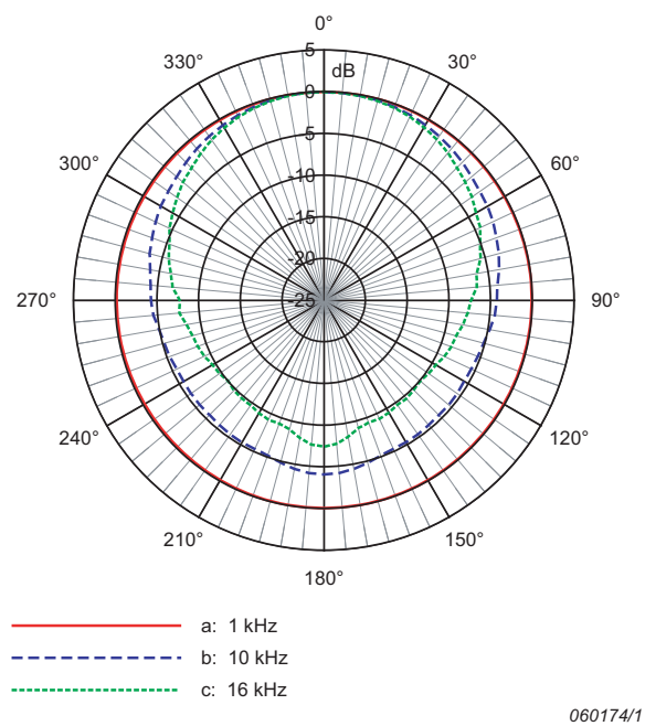
Fig. 3 Typical directivity plot
