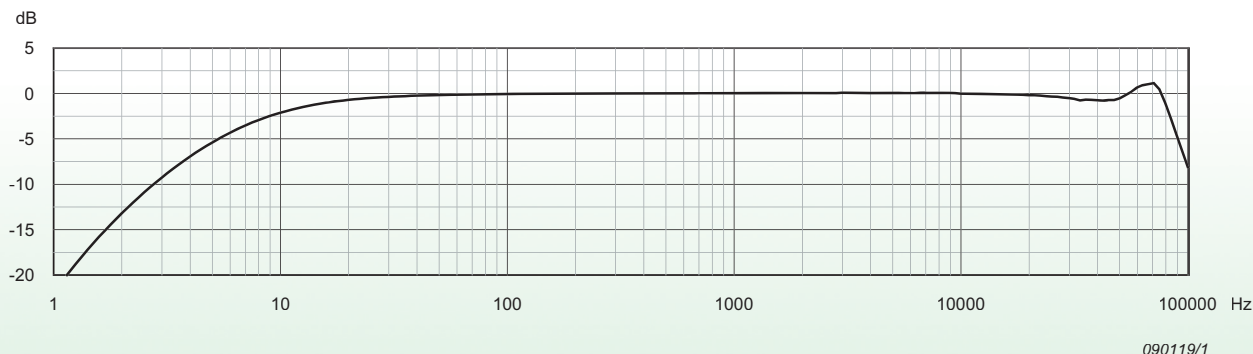
Fig. 1 Type 4944-A pressure-field response without grid
