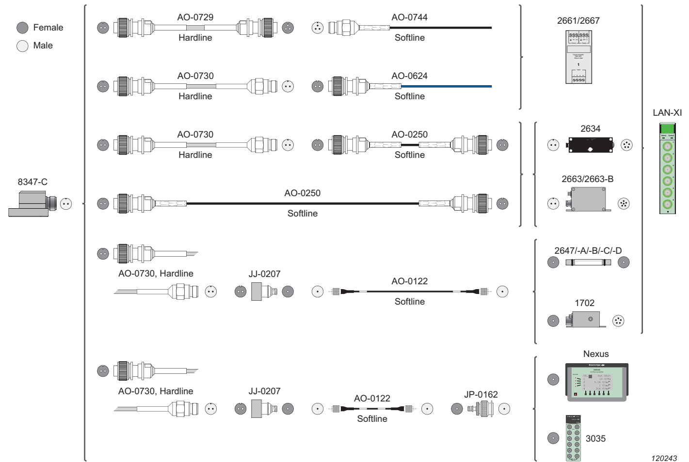
Fig. 2 Typical configurations with Type 8347-C
