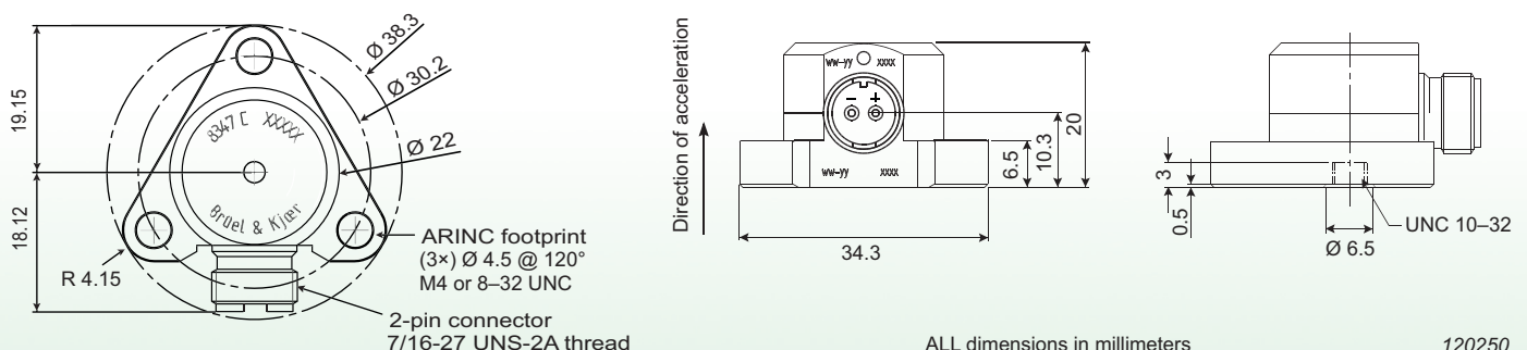
Fig. 1 Outline drawing of Type 8347-C
