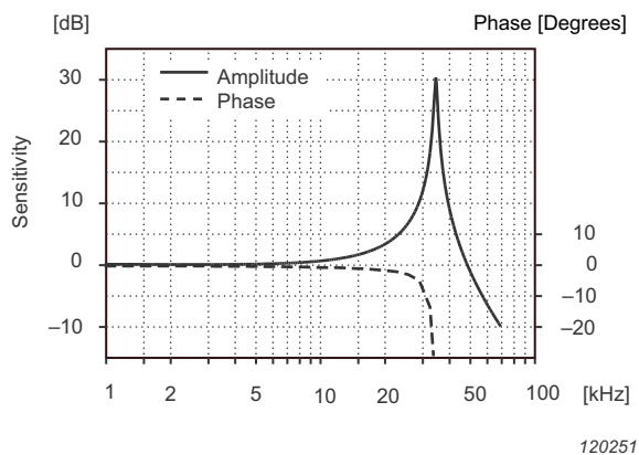
Fig. 3 Typical high frequency response
