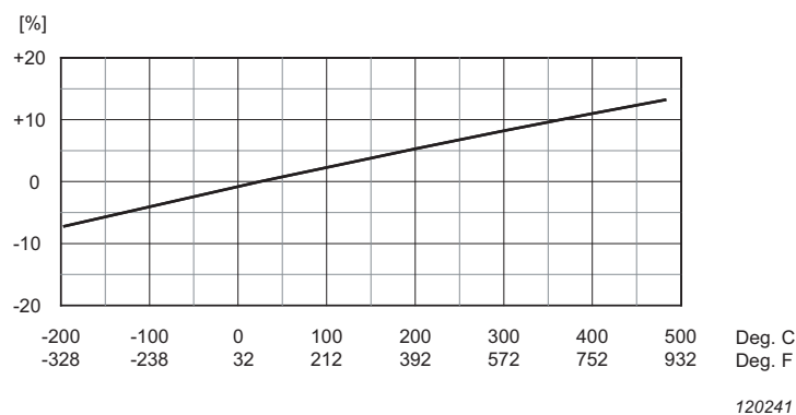
Fig. 4 Sensitivity deviation as a function of temperature
