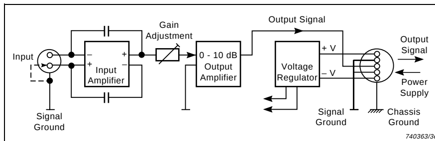
Fig. 1 Simplified block diagram of the Charge Amplifier Type 2634
