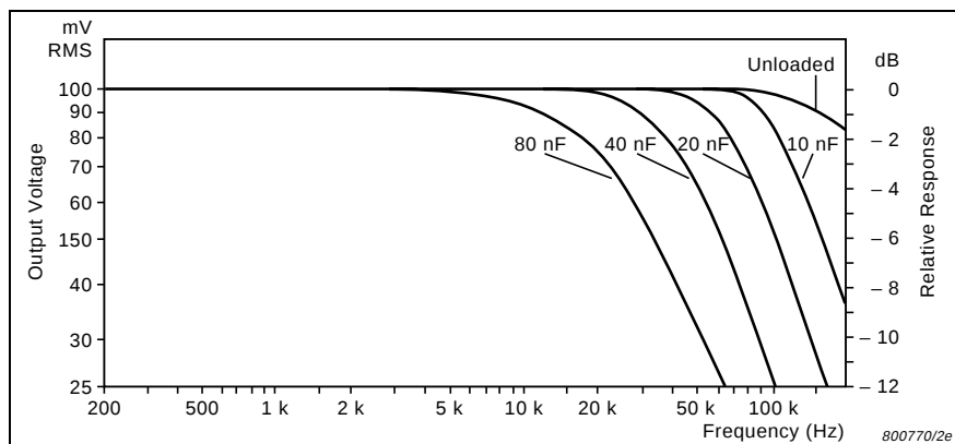
Fig. 2 Typical small signal high frequency response of Type 2634 for different capacity loads at the output. Assuming a cable capacitance of 100 pF/m, a 10 nF load is equivalent to 100 m of cable at the output
